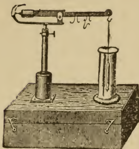
Fig. 83. WESTPHAL'S APPARATUS FOR OBTAINING THE SPECIFIC GRAVITY OF LIQUIDS.
